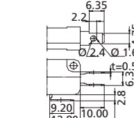
Q187 Quick Connect 187 Series
