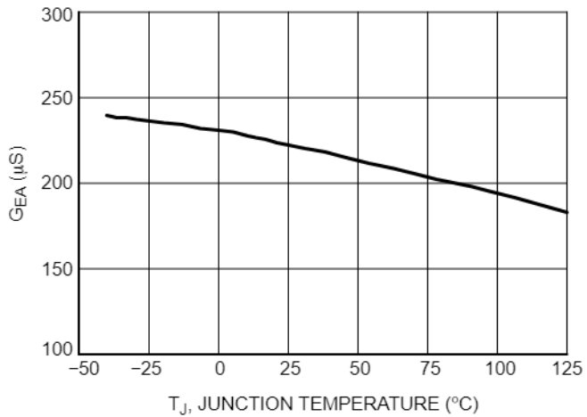
Figure 6. Error Amplifier Gain vs. Temperature
