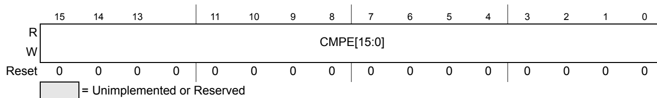
Figure 16-10. ATD Compare Enable Register (ATDCMPE)
