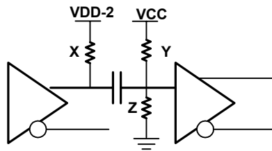
Figure 10. Termination for LVPECL to H I SL interface for V_{CC} = 2.5V would use X = 50\text{ Ohms} , Y = 2300\text{ Ohms} , and Z = 1000\text{ Ohms} . See application note titled PECL Translation, SAW Oscillators, and Specs for Other Signalling Standards and Supplies
