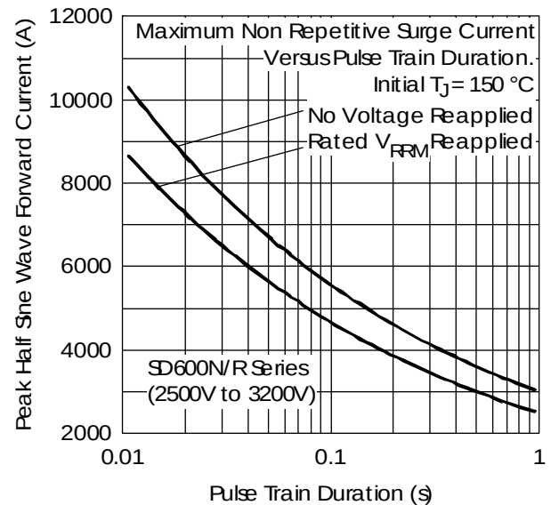
Fig. 12 - Maximum Non-Repetitive Surge Current
