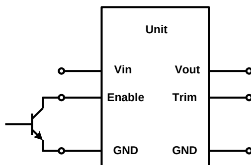
Figure 25: Enable Input drive circuit
