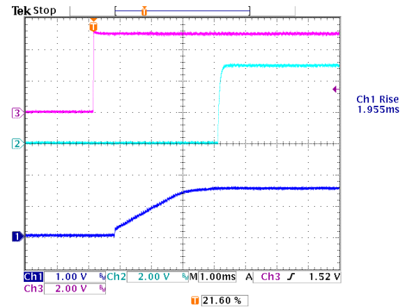
Figure 14: Control Turn on, 1.5V/80A out Ch1: Vo, Ch2:PG, Ch3:Enable
