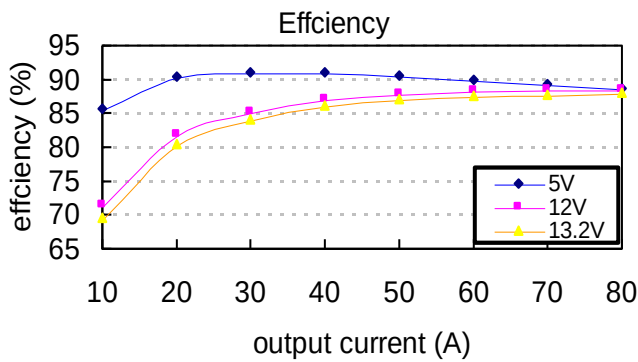
Figure 3: Converter efficiency vs. output current (1.8V output voltage)
