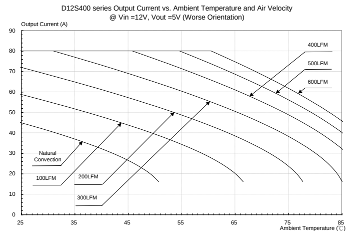
Figure 35: Output current vs. ambient temperature and air velocity @ Vin=12V, Vout=5.0V (Worst Orientation)
