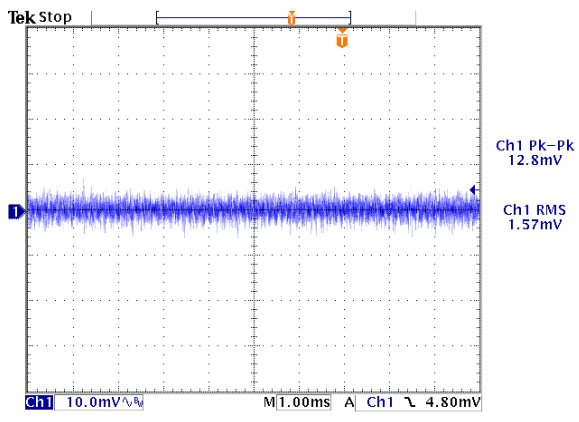
Figure 11: Output ripple & noise at 12Vin, 3.3V/80A out (10mv/div, 1mS/div)
