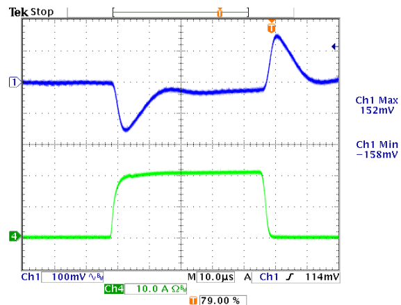
Figure 24: Typical transient response, 5.0V output CH1:Vo, Ch4:I o ,10A/div
