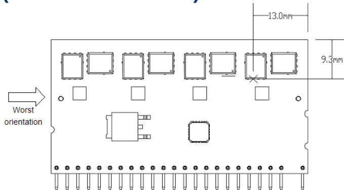
Figure 28: Hot spot temperature measured point
