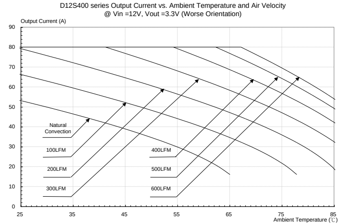
Figure 34: Output current vs. ambient temperature and air velocity @ Vin=12V, Vout=3.3V (Worst Orientation)
