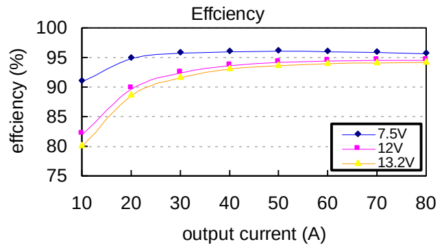
Figure 6: Converter efficiency vs. output current (5.0V output voltage)
