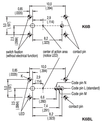
PCB LAYOUT, MOUNTING SIDE
