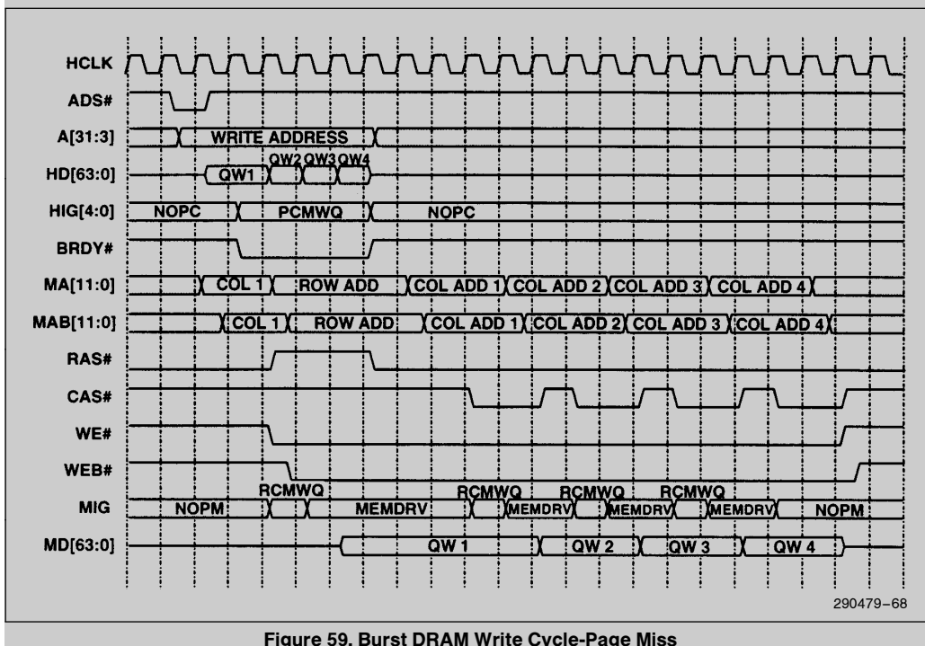
Figure 59. Burst DRAM Write Cycle-Page Miss
