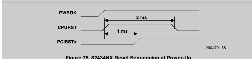
Figure 76. 82434NX Reset Sequencing at Power-Up
