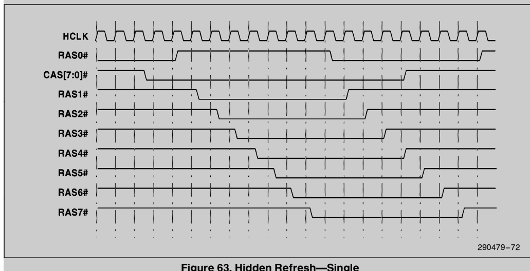
Figure 63. Hidden Refresh—Single
