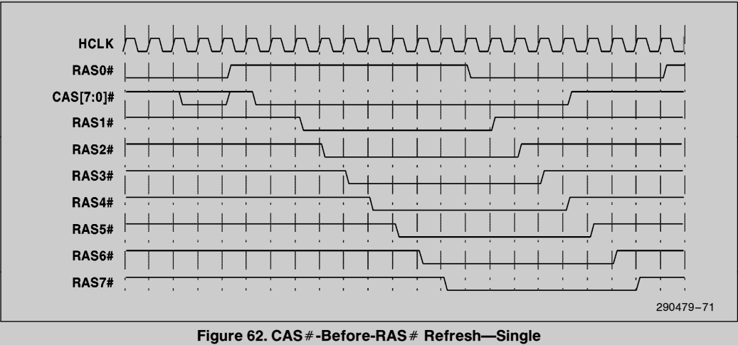
Figure 62. CAS#-Before-RAS# Refresh—Single
