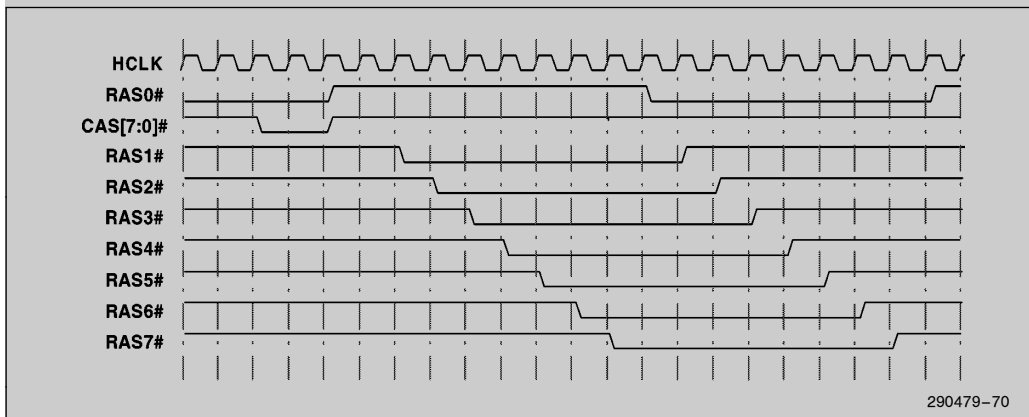
Figure 61. RAS#-Only Refresh—Single
