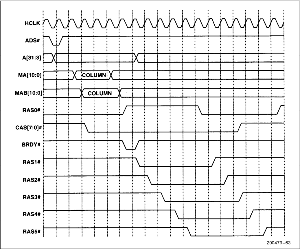
Figure 54. Hidden Refresh-Single
