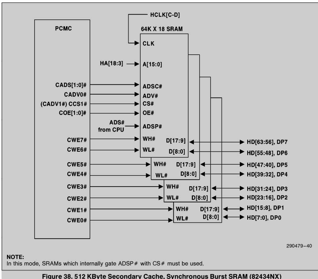
Figure 38. 512 KByte Secondary Cache, Synchronous Burst SRAM (82434NX)
