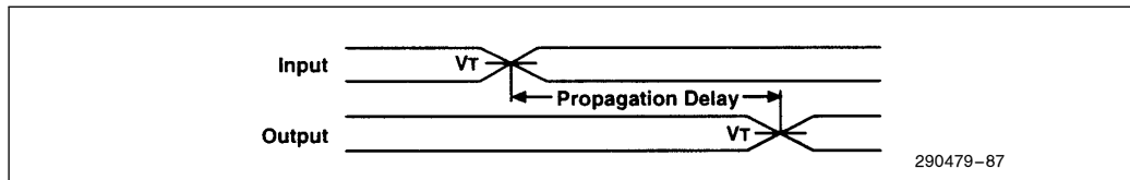
Figure 77. Propagation Delay
