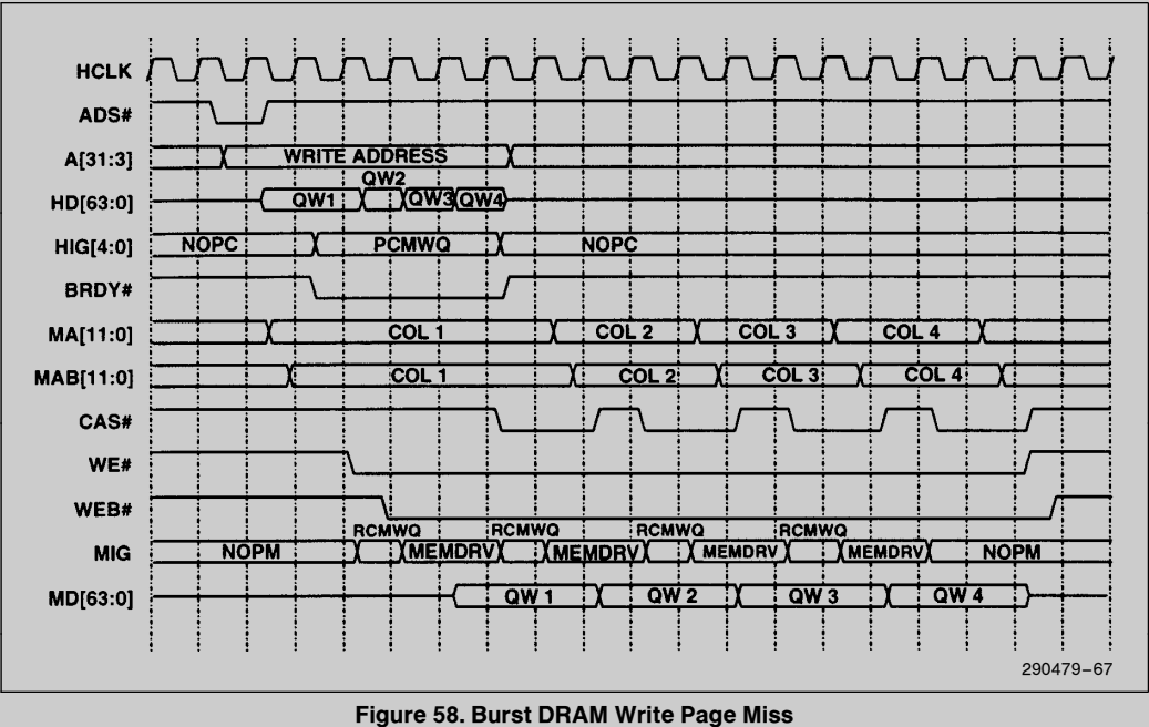
Figure 58. Burst DRAM Write Page Miss
