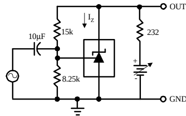
Small Signal Gain and Phase Shift Test Circuit
