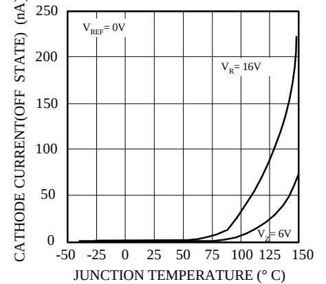
Off State Cathode Current vs. Junction Temperature
