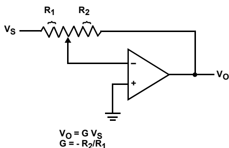
FIGURE 17. INVERTING AMPLIFIER
