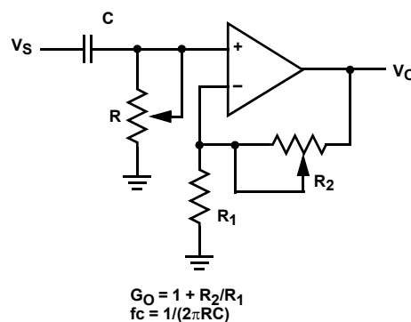
FIGURE 16. FILTER
