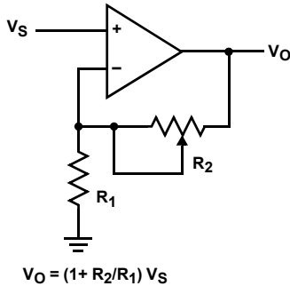
FIGURE 11. NON-INVERTING AMPLIFIER
