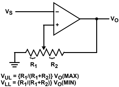
FIGURE 14. COMPARATOR WITH HYSTERESIS
