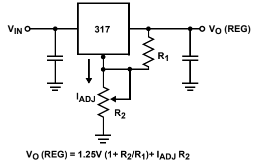
FIGURE 12. VOLTAGE REGULATOR
