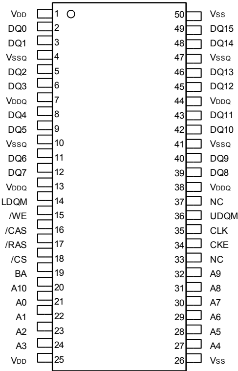
50pin TSOP-II
