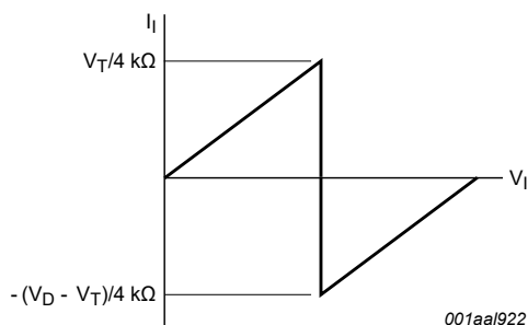
Figure 9. Typical input current versus input voltage graph
