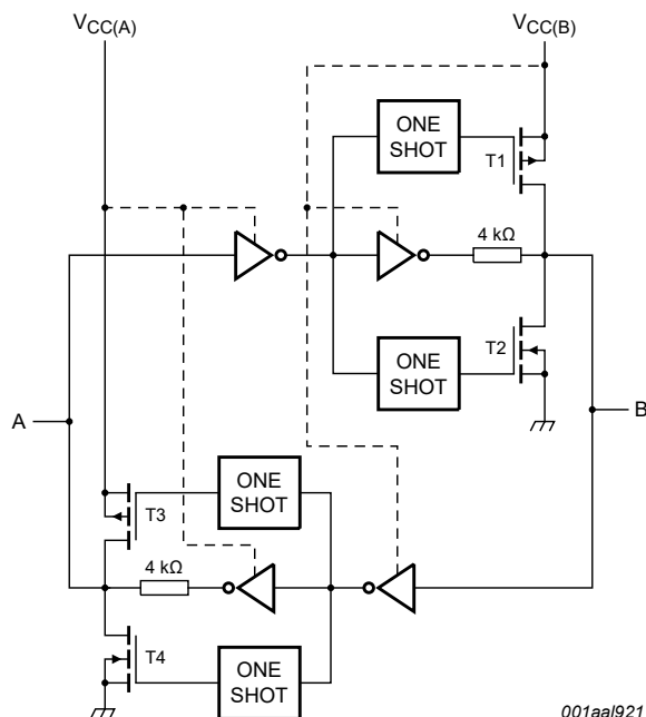
Figure 8. Architecture of NTB0102 I/O cell (one channel)
