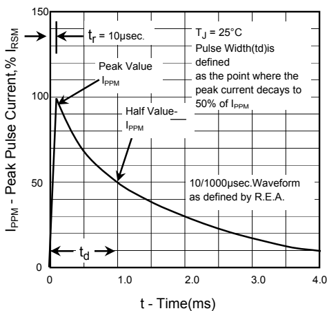
Fig.3 Pulse Waveform
