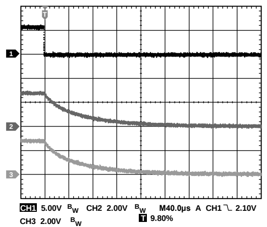
Figure 27. Shutdown Response, ADP221
