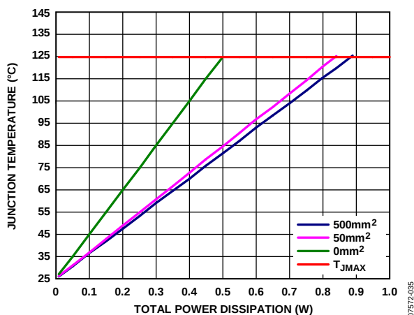
Figure 35. Junction Temperature vs. Total Power Dissipation, T_A = 25^\circ\text{C}
