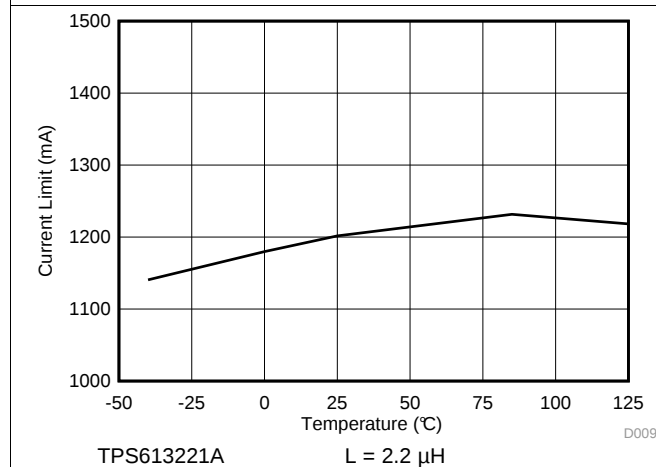
Figure 11. Current Limit with Different Temperature
