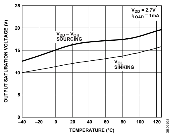
Figure 25. Output Saturation Voltage vs. Temperature
