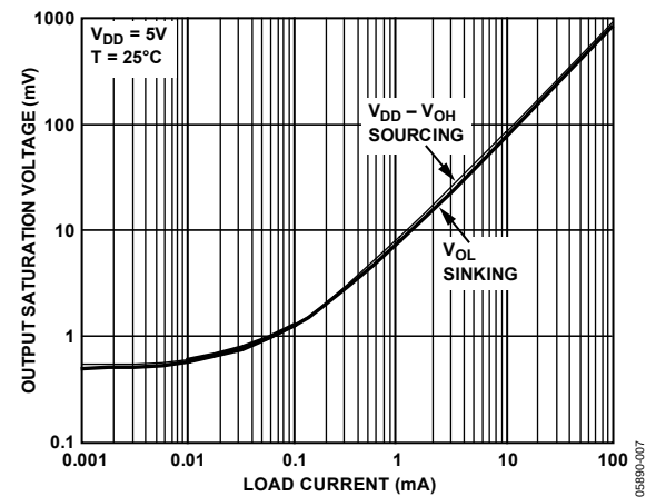
Figure 7. Output Saturation Voltage vs. Load Current
