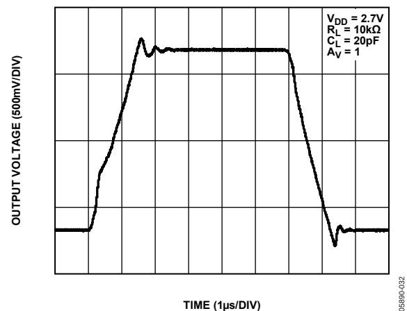
Figure 32. Large-Signal Transient Response
