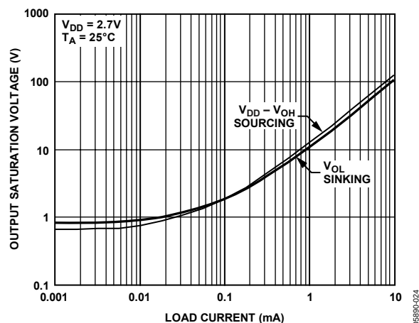
Figure 24. Output Saturation Voltage vs. Load Current
