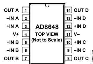
Figure 2. 14-Lead SOIC (R-14)
