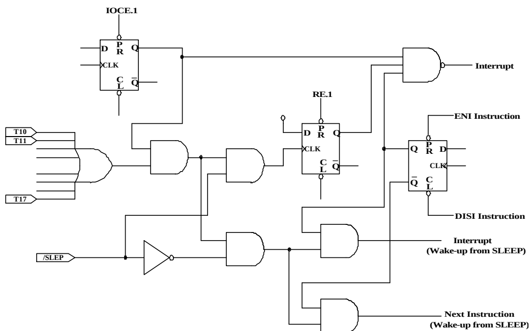
Fig. 8 The Circuit of I/O Port and I/O Control Register for P61~P67
