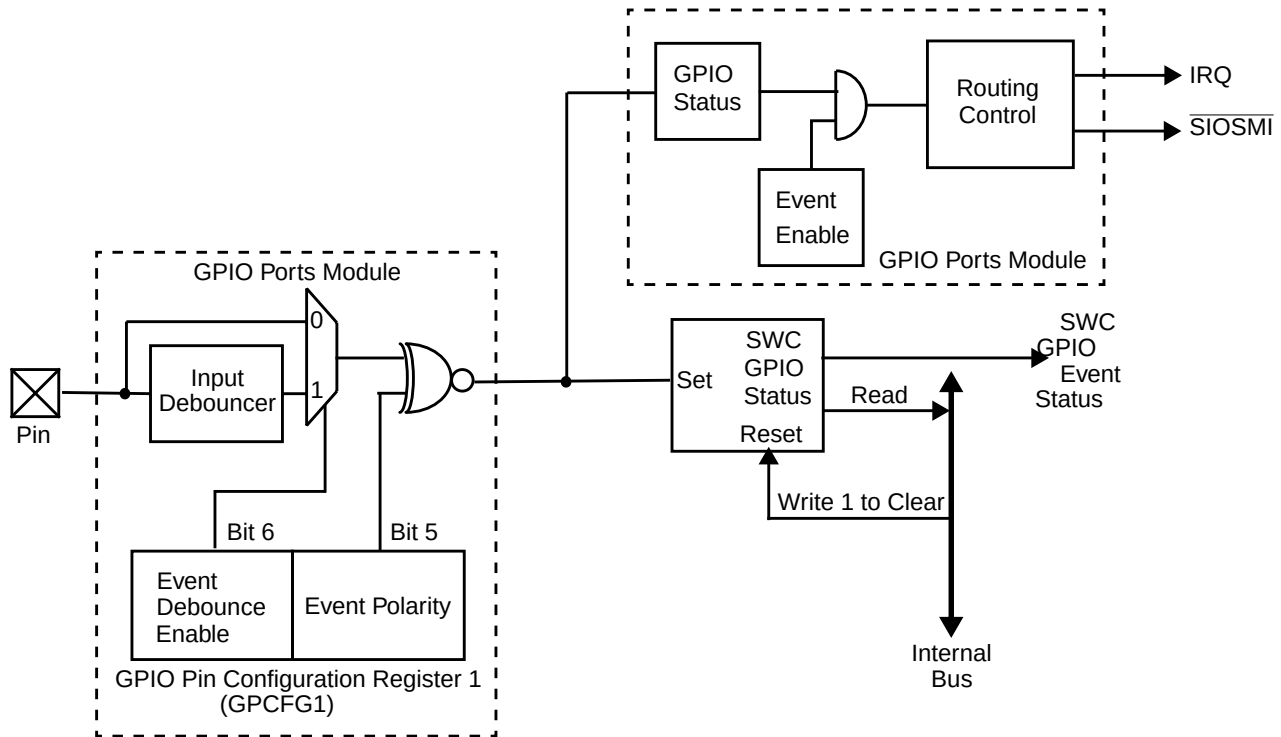
Figure 48. GPIO Events
