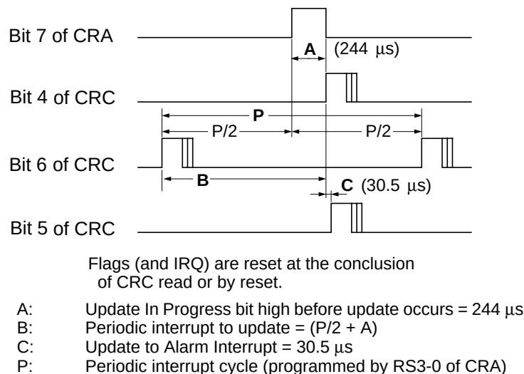
Figure 46. Interrupt/Status Timing
