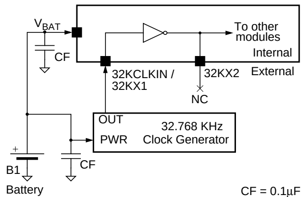
Figure 40. External Oscillator Connections
