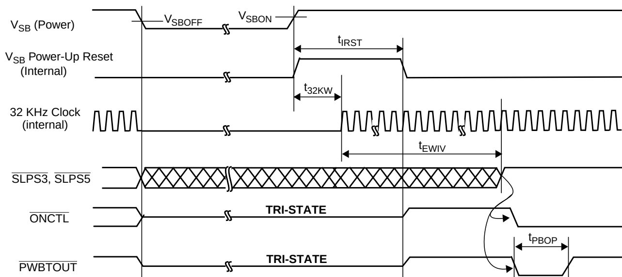
Figure 68. Resume by \overline{\text{SLPS3}} , \overline{\text{SLPS5}} , After Power Fail (No V_{BAT} )
