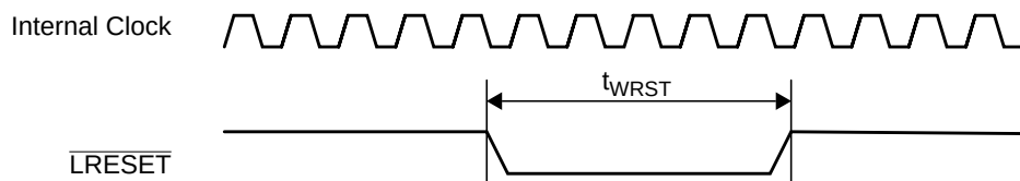
Figure 59. Hardware Reset
