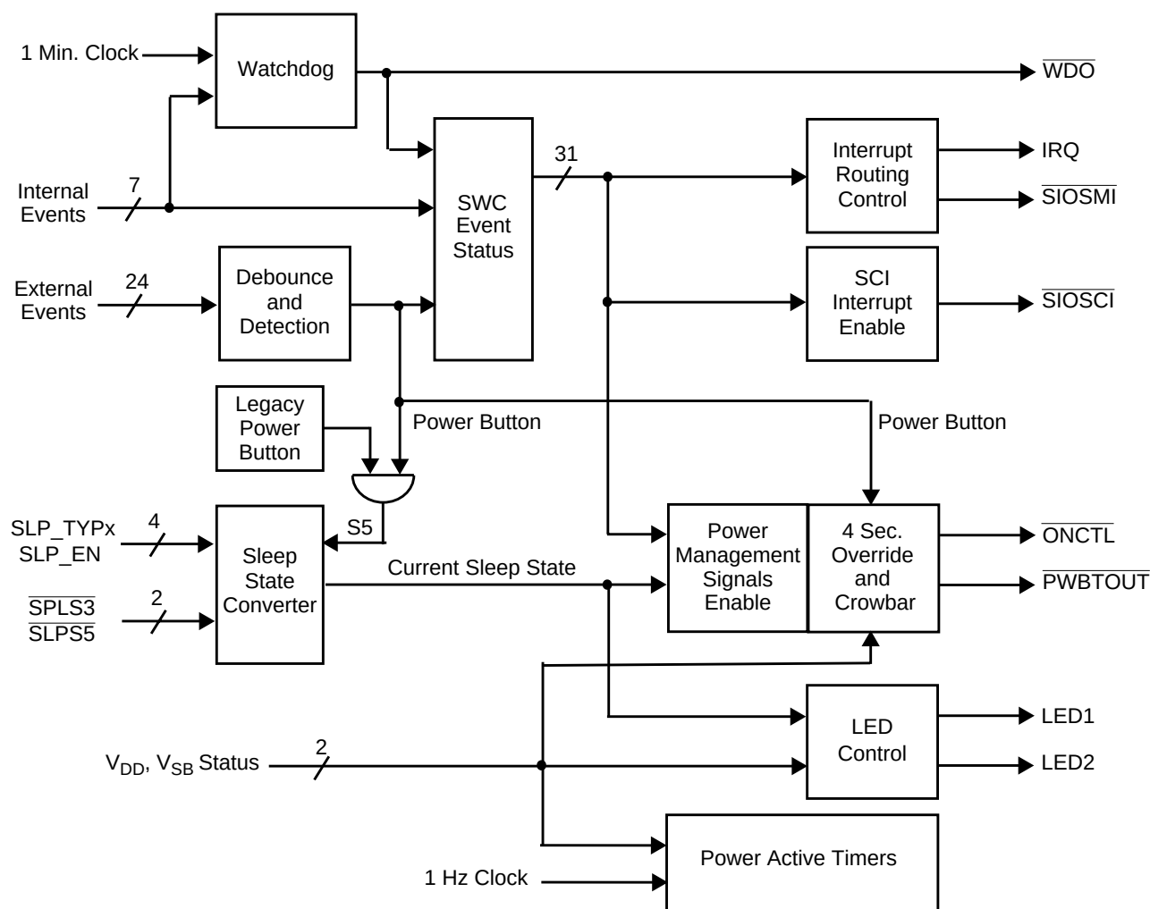
Figure 47. SWC Block Diagram
