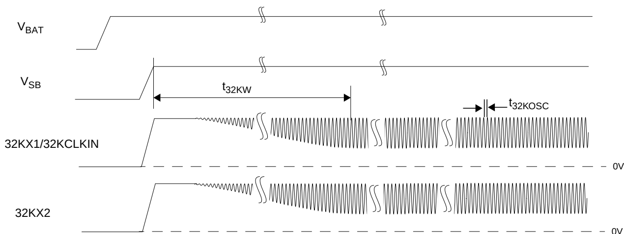
Figure 61. Low Frequency Clock Waveforms
