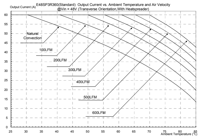
Figure 23: Output current vs. ambient temperature and air velocity @Vin=48V(Transverse Orientation, with heat spreader)
