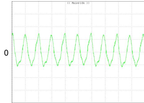
Figure 11: Input Terminal Ripple Current, i_c , at full rated output current and nominal input voltage with 12µH source impedance and 100µF electrolytic capacitor (200 mA/div, 2us/div)
