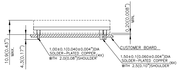
SIDE VIEW
