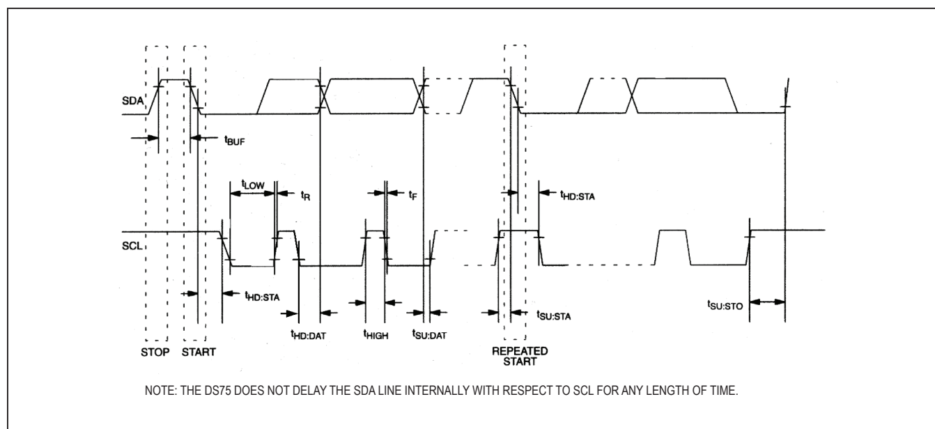
Figure 2. Timing Diagram
