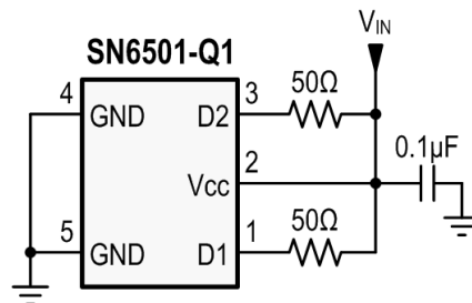
图 36. Test Circuit For R_{ON} , F_{SW} , F_{St} , T_{r-D} , T_{f-D} , T_{BBM}
