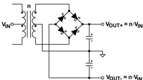
图 46. Bridge Rectifier With Center-Tapped Secondary Enables Bipolar Outputs
