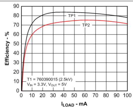
图 10. Efficiency vs Load Current
