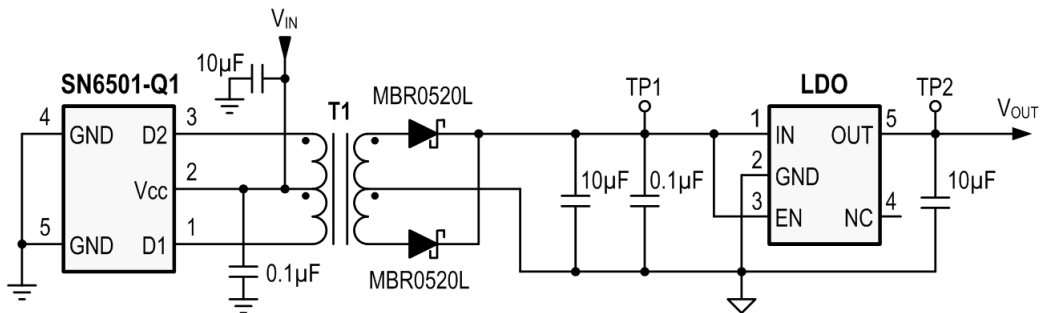
图 35. Measurement Circuit for regulated Output (TP1 and TP2)
