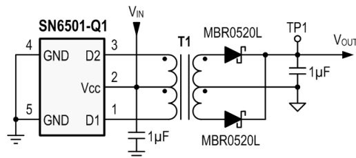
图 44. Unregulated Output for Low-Current Loads With Wide Supply Range
