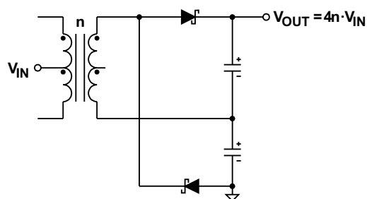
图 49. Half-Wave Rectifier Without Centered Ground and Center-Tapped Secondary Performs Voltage Doubling Twice, Hence Quadrupling V_{IN}
