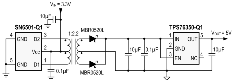
图 41. Typical Application Schematic (SN6501-Q1)
