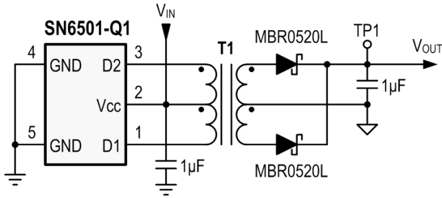
图 33. Measurement Circuit for Unregulated Output (TP1)
