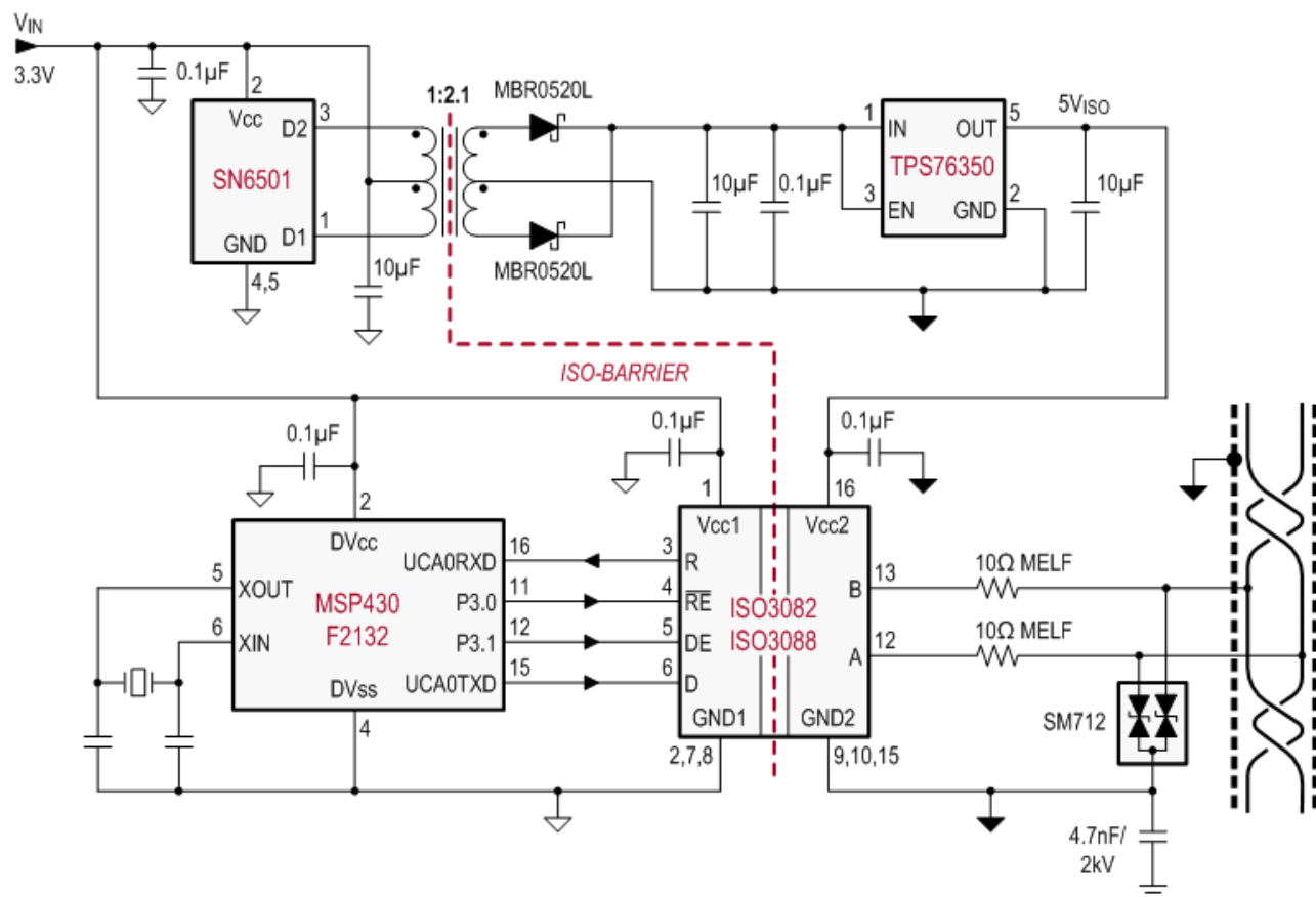
图 50. Isolated RS-485 Interface
