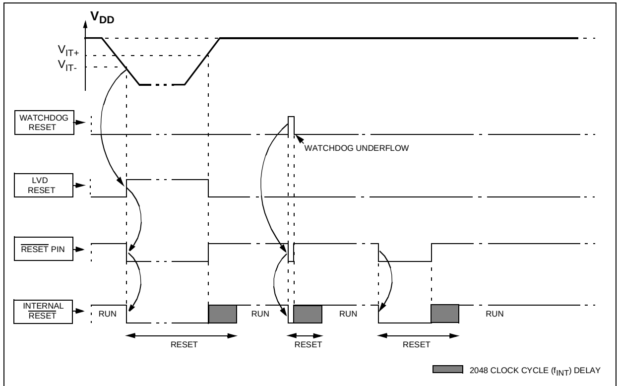
Figure 13. RESET Sequence
