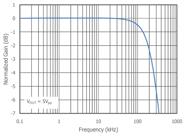
Figure 11: AC Response of Figure 10 ( V_S=10V , R_L=630\Omega )
