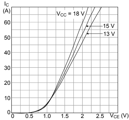
Figure 11. Output characteristics ( T_J = 25^\circ\text{C} )
