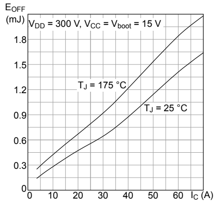
Figure 15. E_{OFF} switching energy vs collector current
