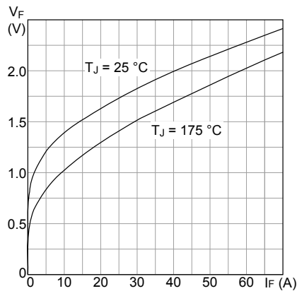
Figure 13. Diode V_F vs forward current
