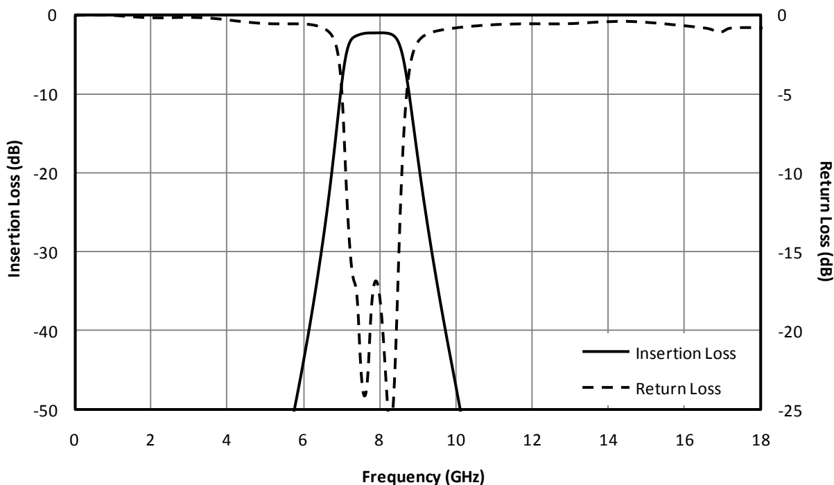
Fig. 1. Magnitude response for a typical FB-0785SM, measured in a connectorized fixture.
