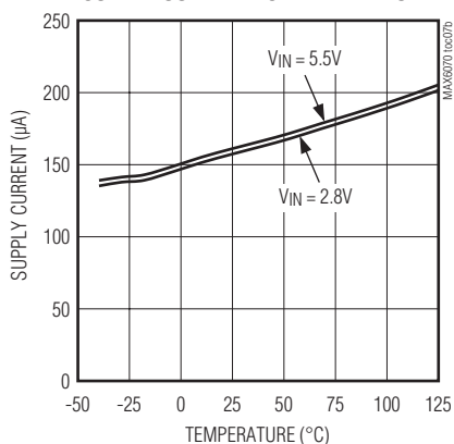
MAX6071_25 SUPPLY CURRENT vs. TEMPERATURE
