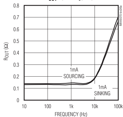
MAX6071_12 R OUT vs. FREQUENCY
