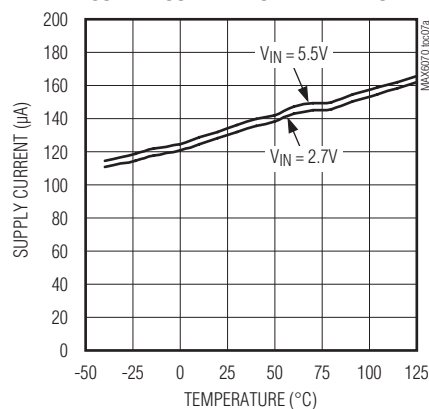
MAX6071_12 SUPPLY CURRENT vs. TEMPERATURE
