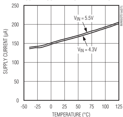
MAX6071_41 SUPPLY CURRENT vs. TEMPERATURE
