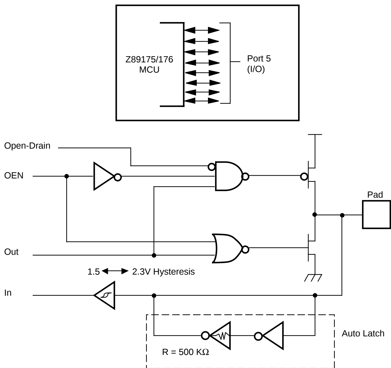
Figure 16. Port 5 Configuration
