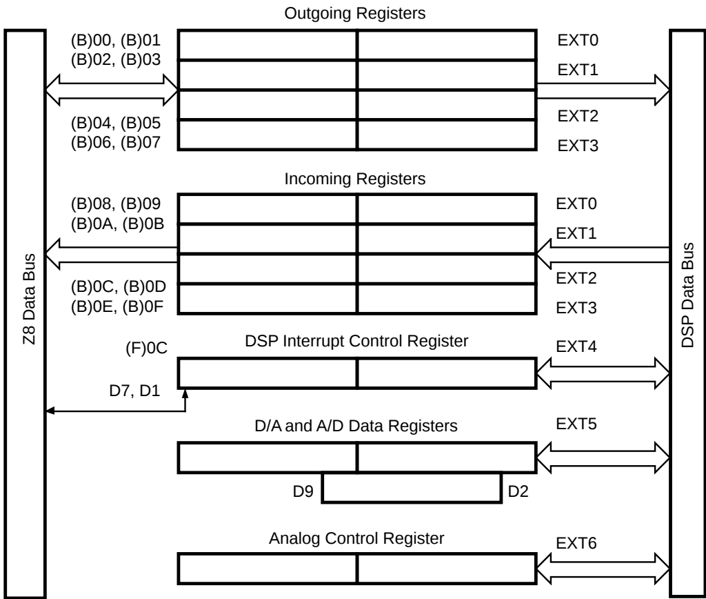
Figure 31. Z8-DSP Interface
