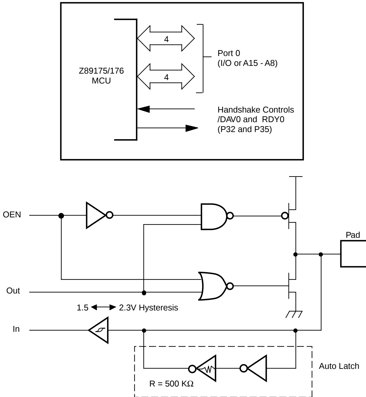
Figure 11. Port 0 Configuration
