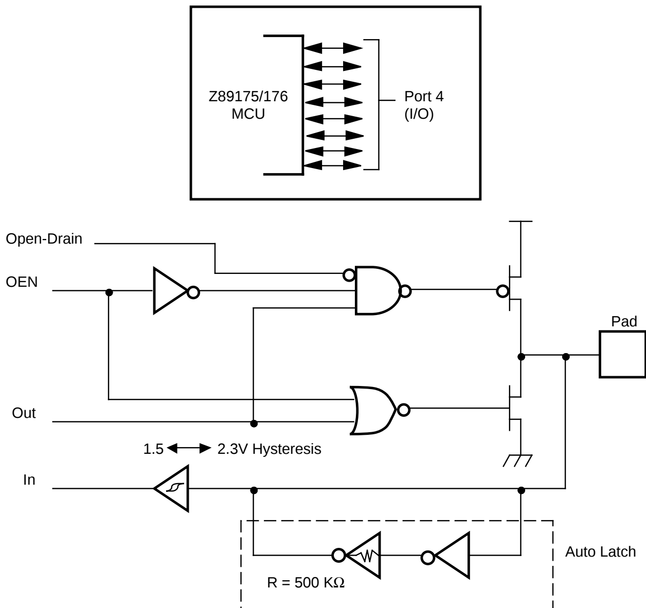
Figure 15. Port 4 Configuration
