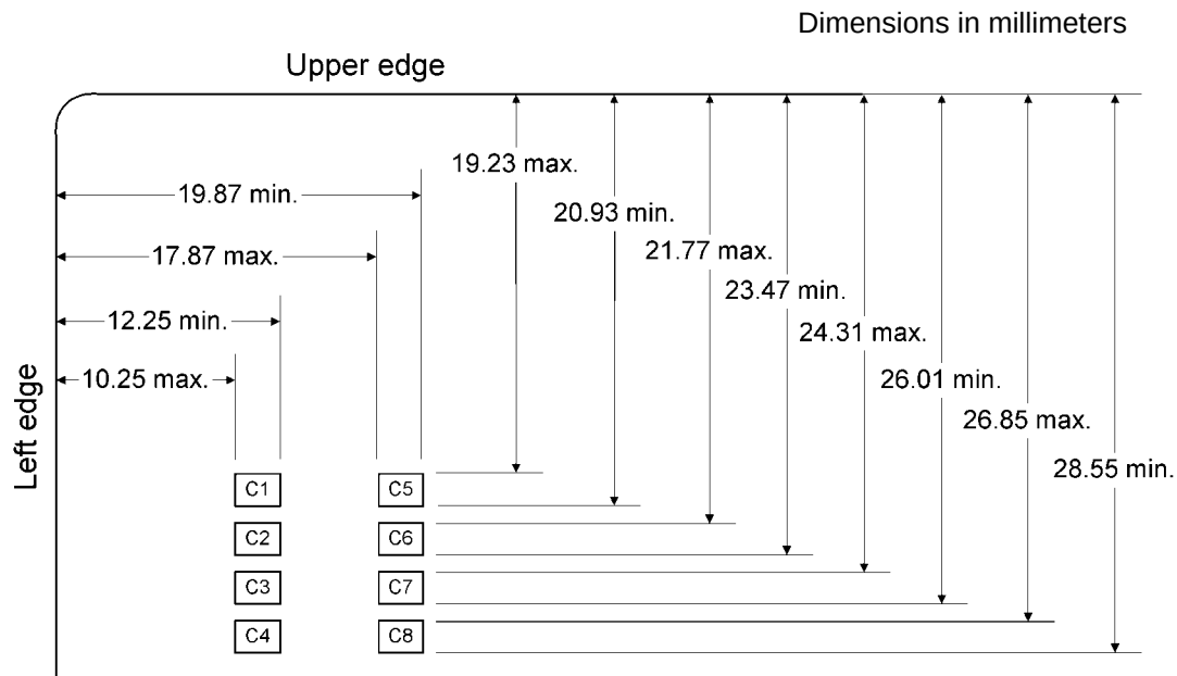
Figure 2. Contacts location
