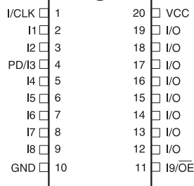
DIP/SOIC
