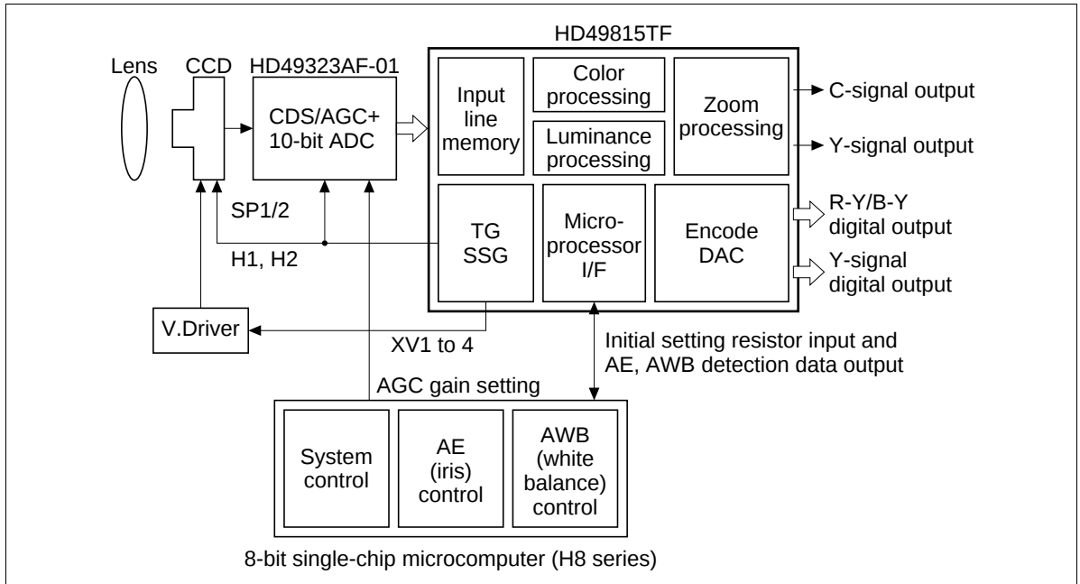
Figure 2 System Configuration
