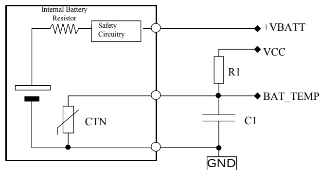
Figure 9 : Connection examples
