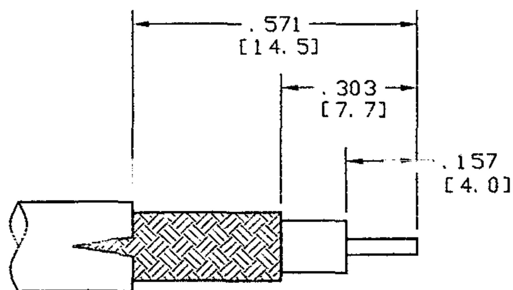
RECOMMENDED CABLE STRIPPING DIM'S
