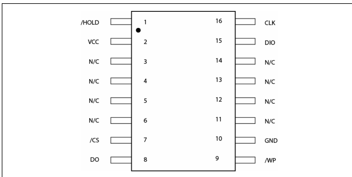
Figure 1d. W25X64 Pin Assignments, 16-pin SOIC 300-mil
