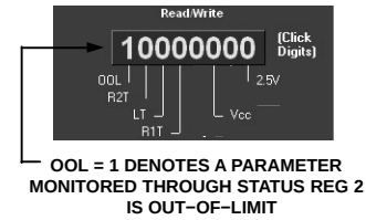
Figure 32. Status Register 1
