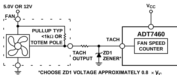
Figure 49. Fan with Strong TACH Pullup to > V_{CC} or Totem-Pole Output, Clamped with Zener and Resistor
