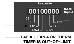
Figure 33. Status Register 2
