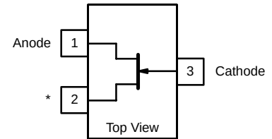
TO-236 (SOT-23)
