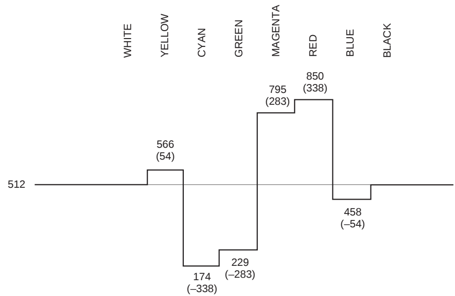
Color Difference (V) Video Output Waveform
