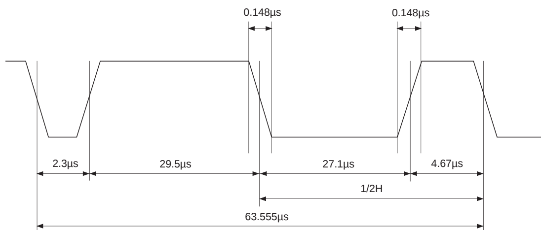
NTSC Equalizing &amp; Synchronizing Pulses
