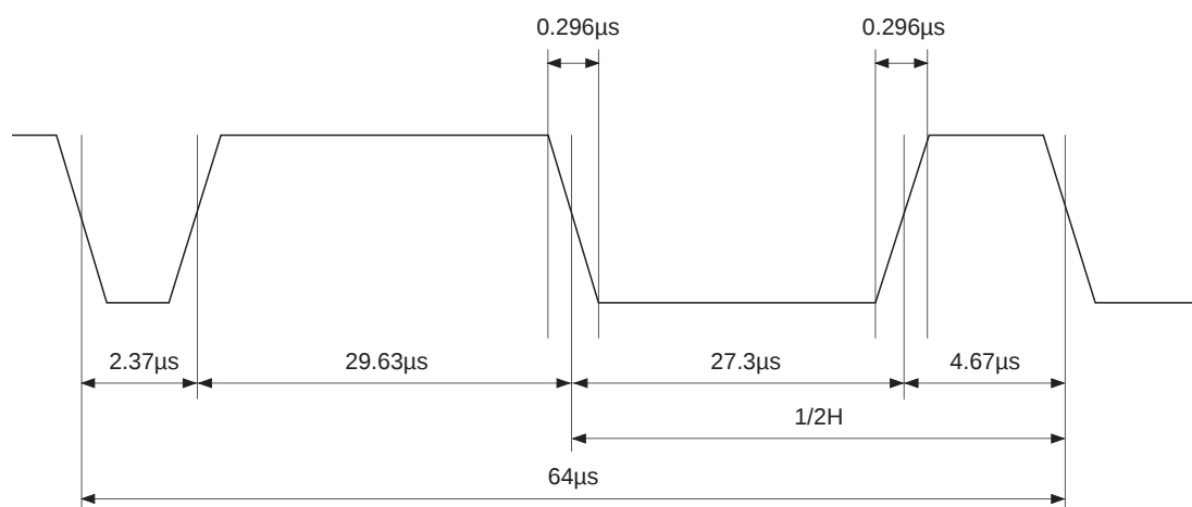
PAL Equalizing &amp; Synchronizing Pulses
