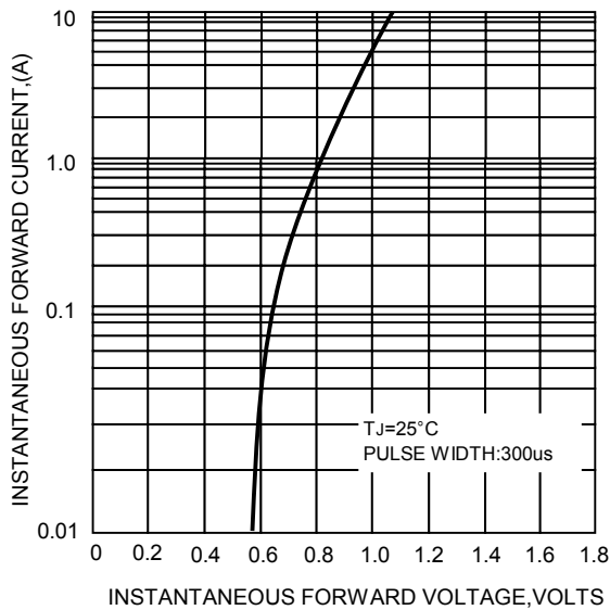
FIG.4-TYPICAL FORWARD CHARACTERISTICS
