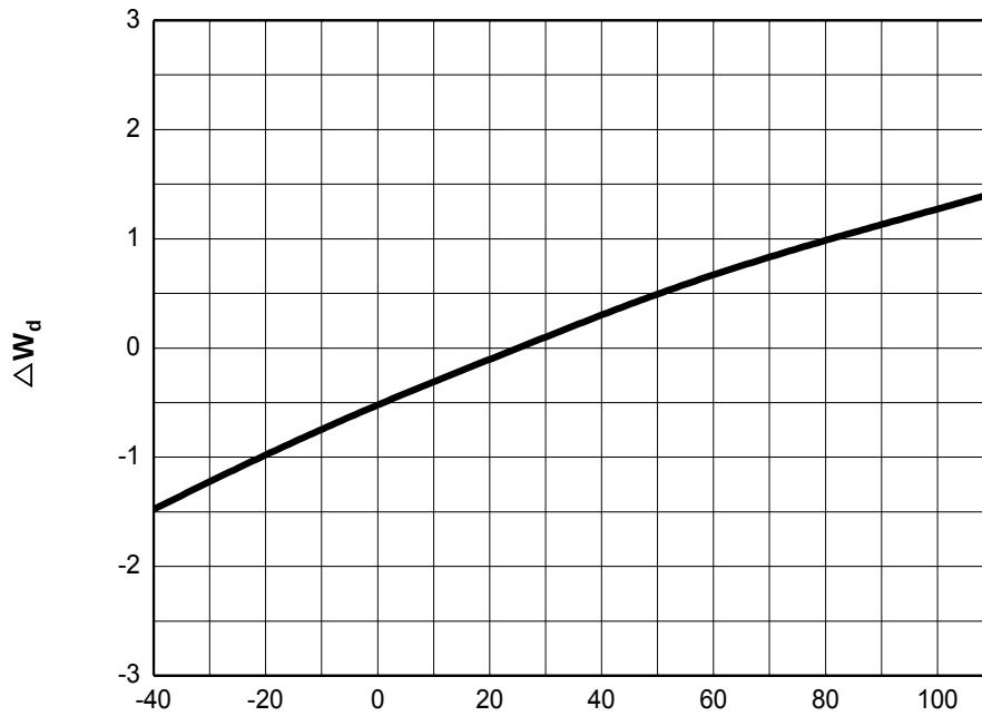
Fig 8. Dominant wavelength shift vs. Junction Temperature, I_F = 10\text{mA}
