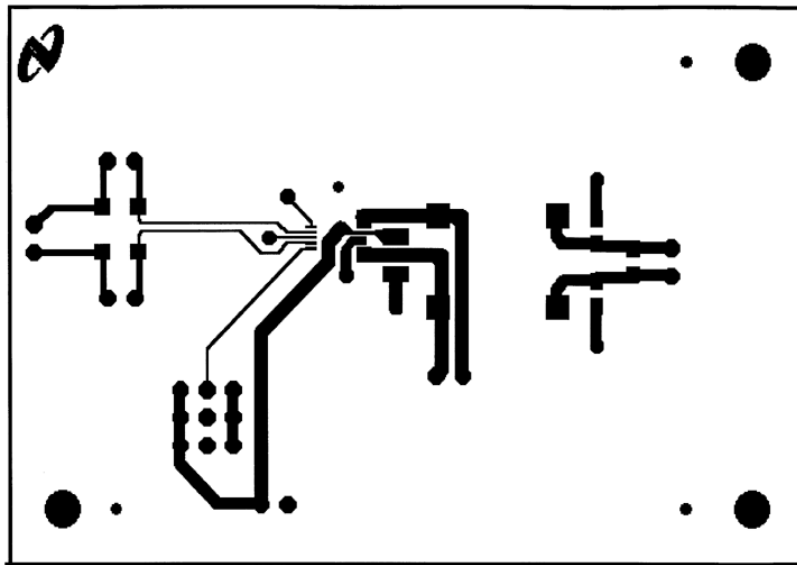
Figure 38. Top Layer
