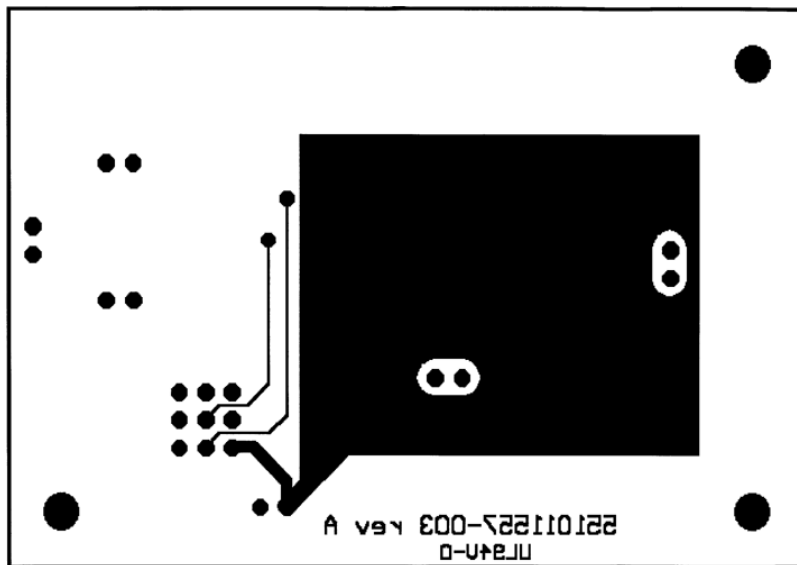
Figure 39. Bottom Layer
