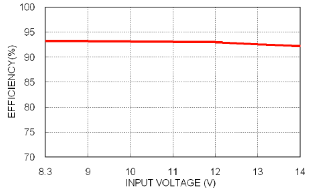
POLS10-12T, Vout=3.3V Efficiency vs. Input Voltage
