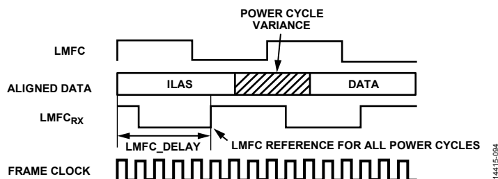
Figure 102. LMFC_DELAY_x to Compensate for Link Delay > LMFC
