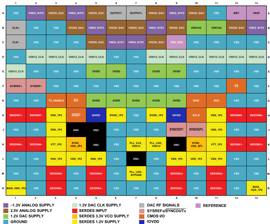
Figure 4. 169-Ball CSP_BGA Pin Configuration
