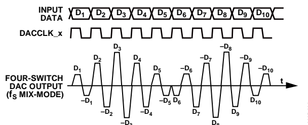
Figure 128. Mix-Mode Waveform
