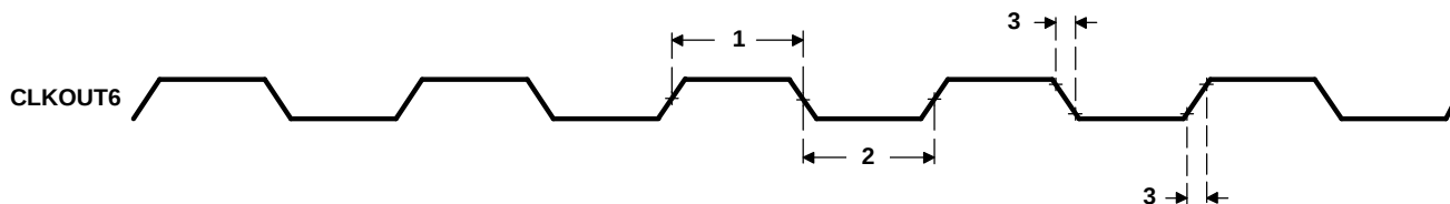
Figure 5-13. CLKOUT6 Timing
