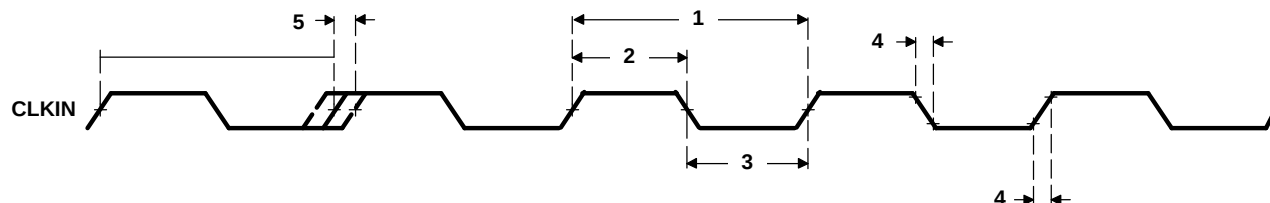
Figure 5-11. CLKIN Timing
