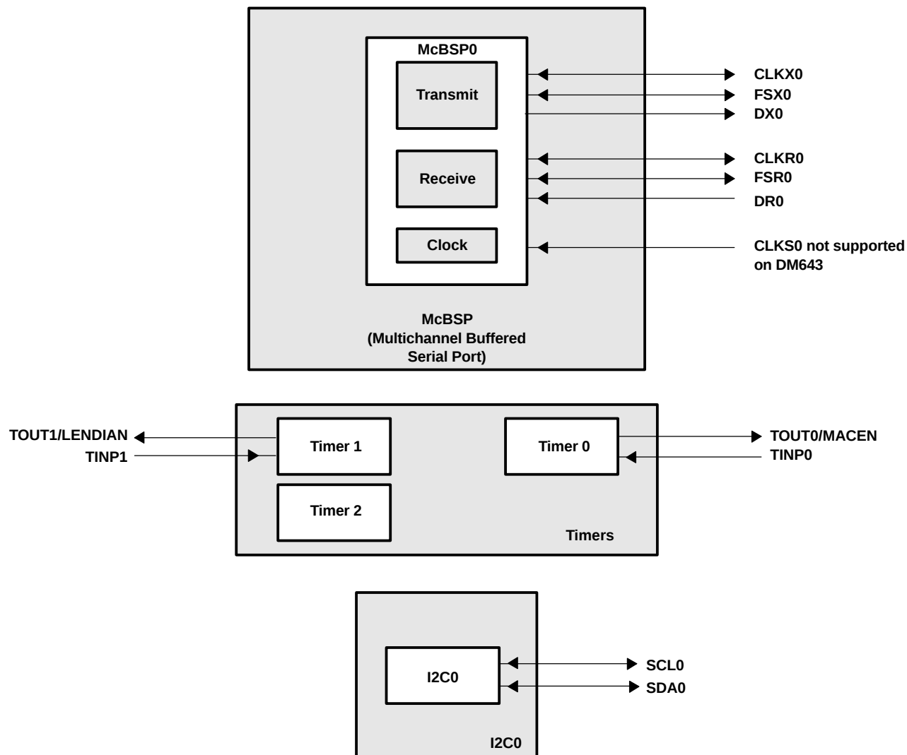
Figure 2-10. McBSP/Timer/I2C0 Peripheral Signals
