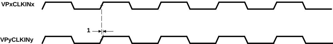
Figure 5-55. Video Port Dual-Display Sync Timing
