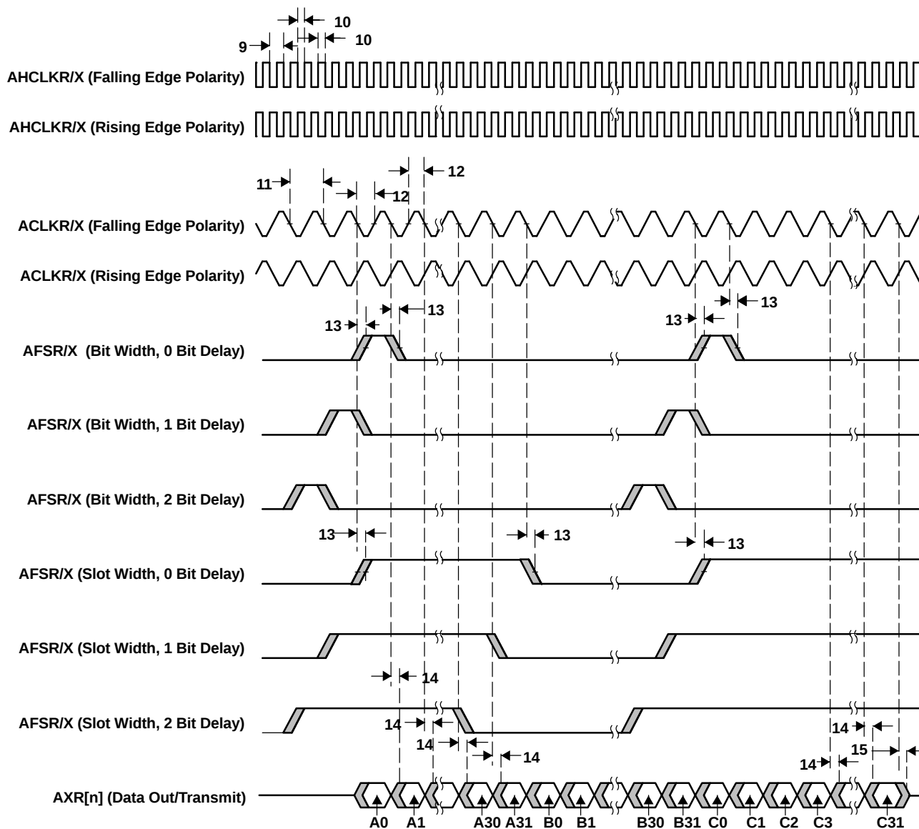
Figure 5-34. McASP Output Timings
