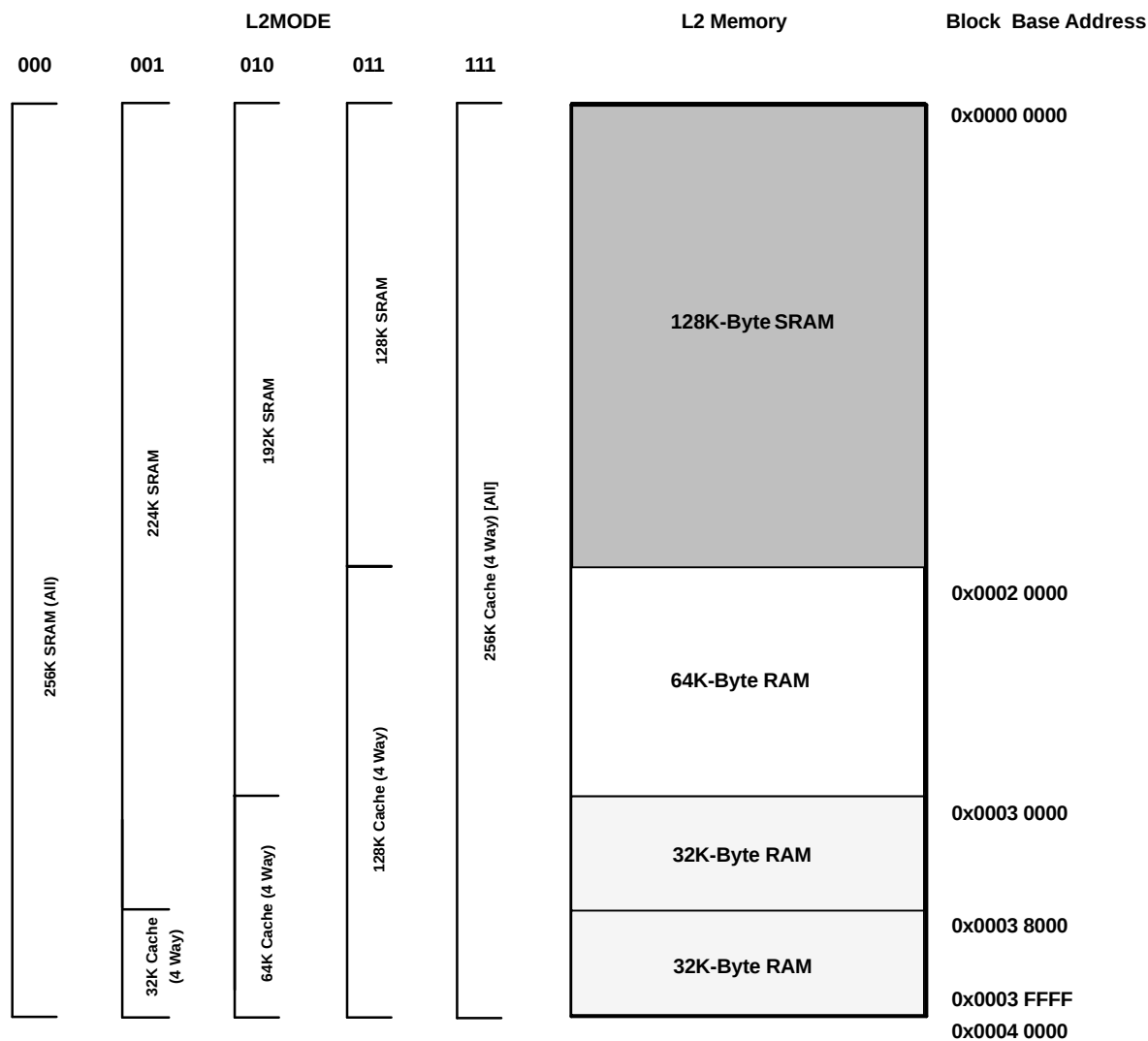
Figure 2-2. TMS320DM643 L2 Architecture Memory Configuration
