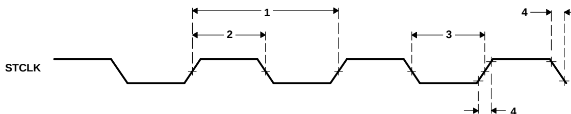
Figure 5-56. STCLK Timing
