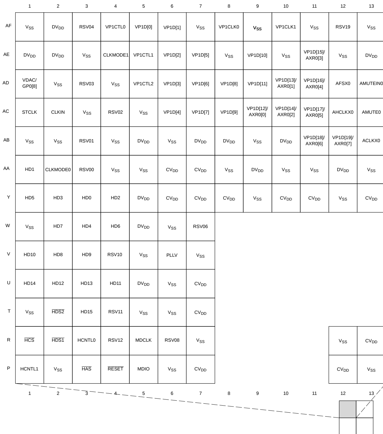
Figure 2-3. DM643 Pin Map [Quadrant A]
