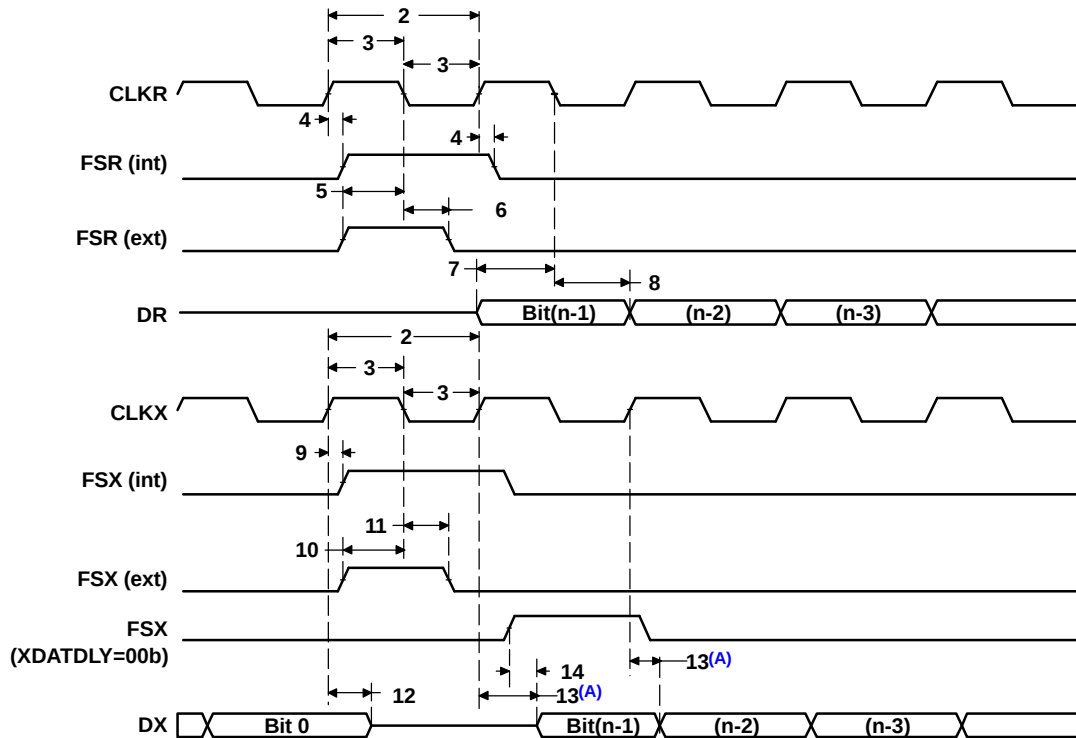
Figure 5-46. McBSP Timing
