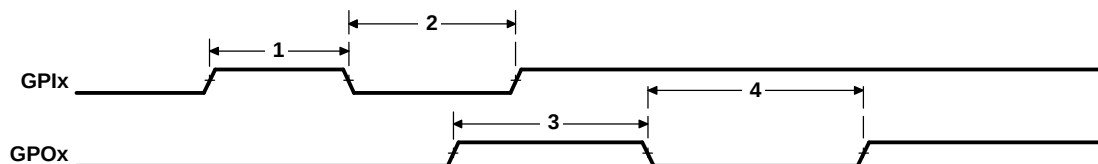
Figure 5-66. GPIO Port Timing
