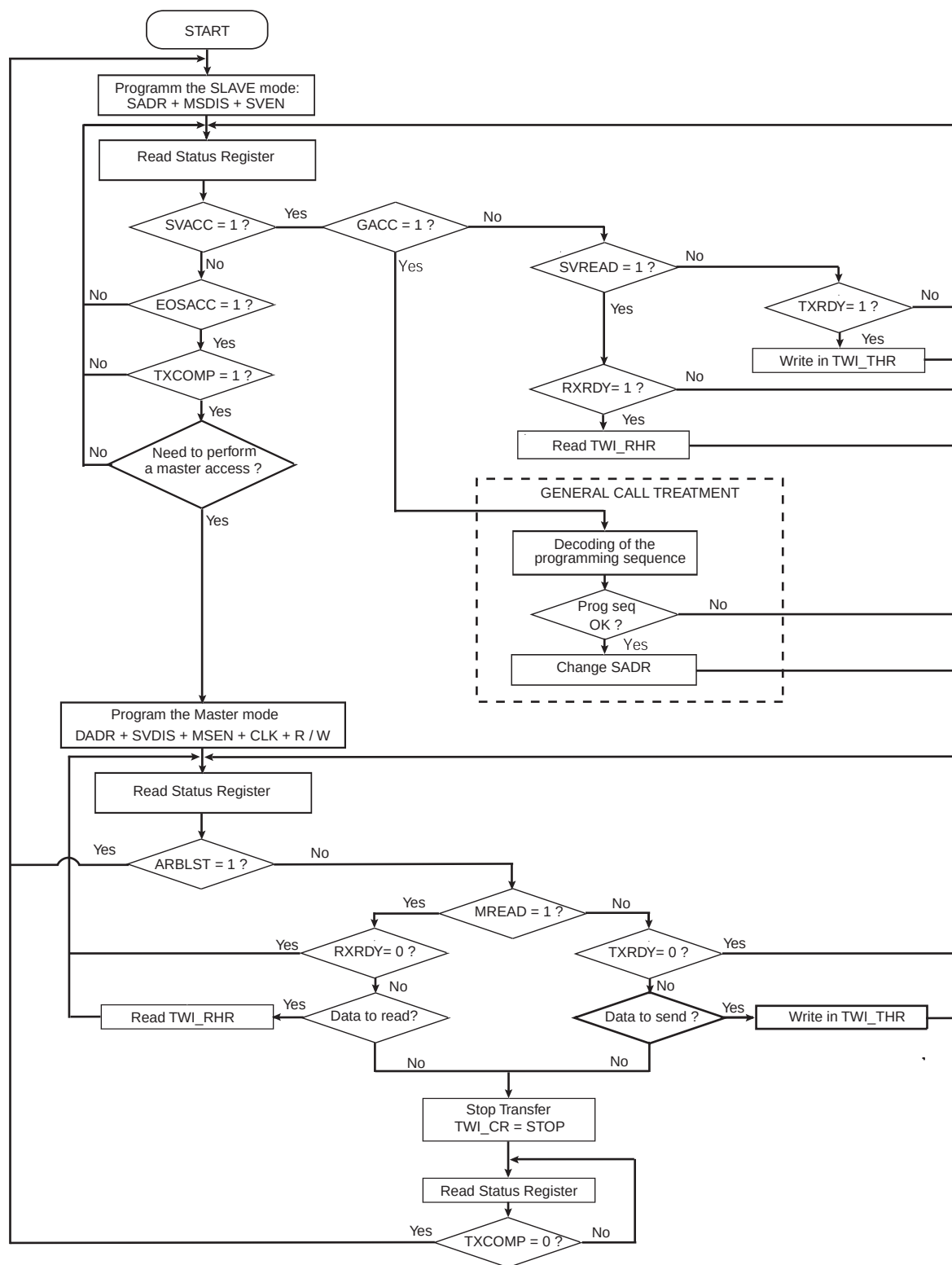
Figure 33-23. Multi-master Flowchart
