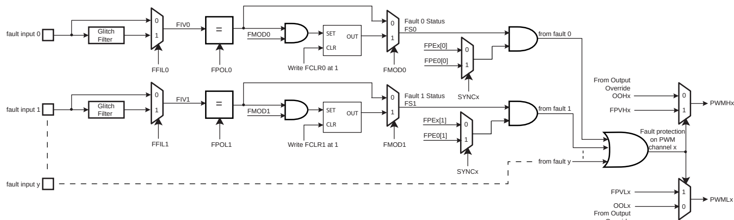
Figure 38-9. Fault Protection
