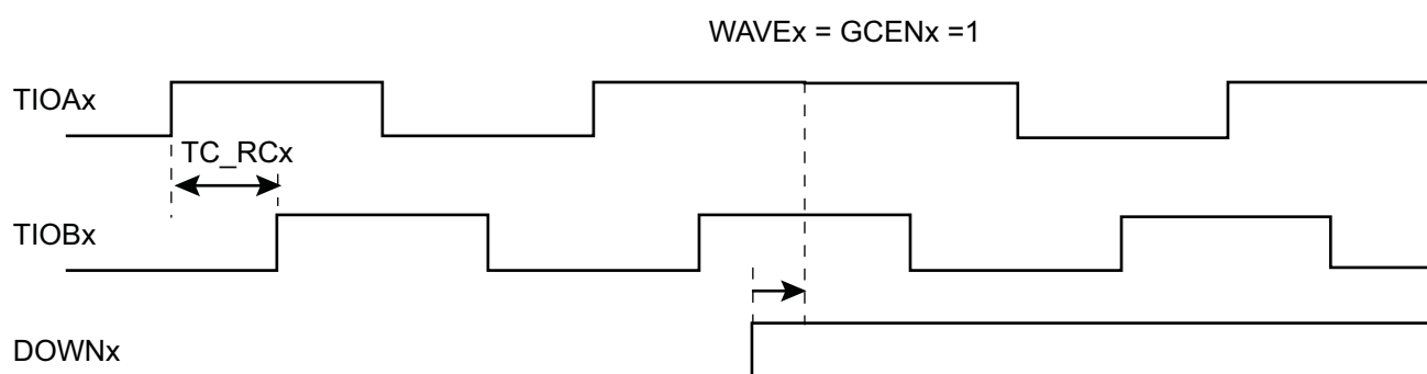
Figure 36-20. 2-bit Gray Up/Down Counter
