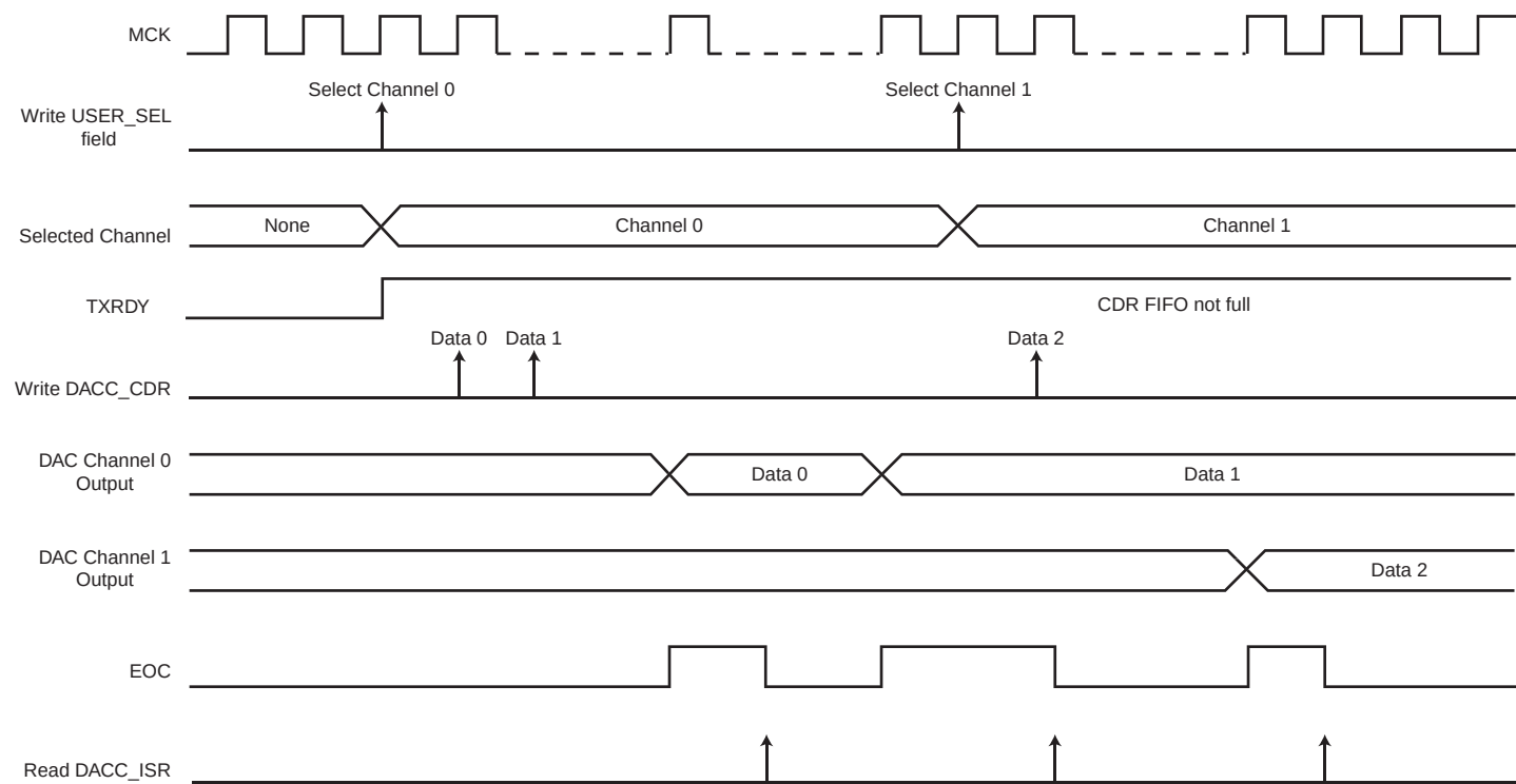
Figure 44-2. Conversion Sequence
