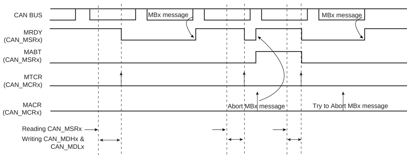
Figure 40-15. Transmitting Messages
