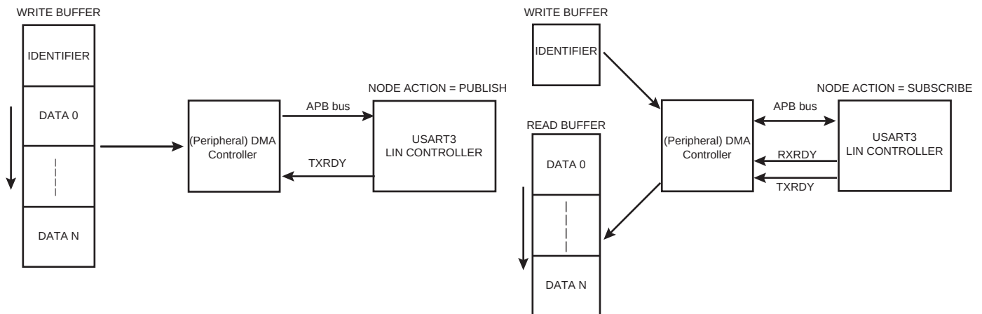
Figure 35-53. Master Node with PDC (PDCM = 0)
