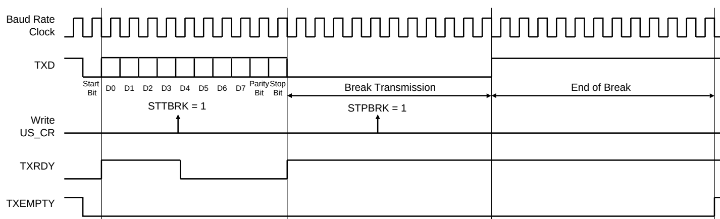
Figure 35-26. Break Transmission
