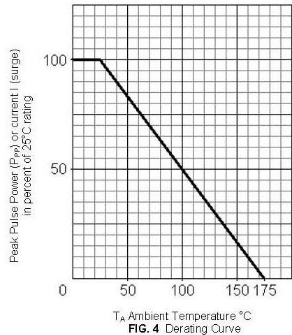
FIG. 4 Derating Curve
