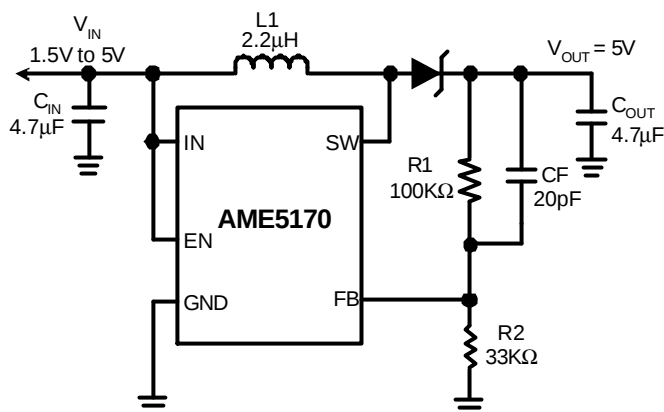
Figure.1 Typical 5V Application
