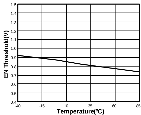
EN Thershold Low vs. Temperature
