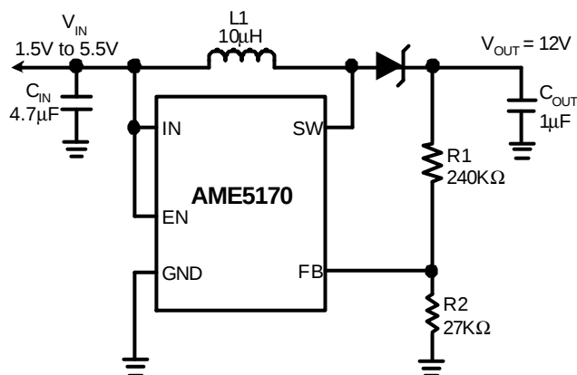
Figure.2 Typical 12V Application
