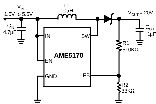
Figure.3 Typical 20V Application
