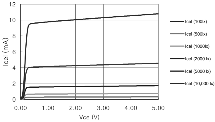
Collector current Vs. Collector - Emitter voltage T_a=25^\circ
