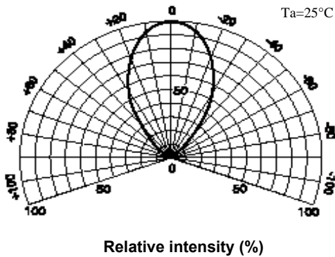
Radiant Pattern Angle (deg.) T_a=25^\circ C
