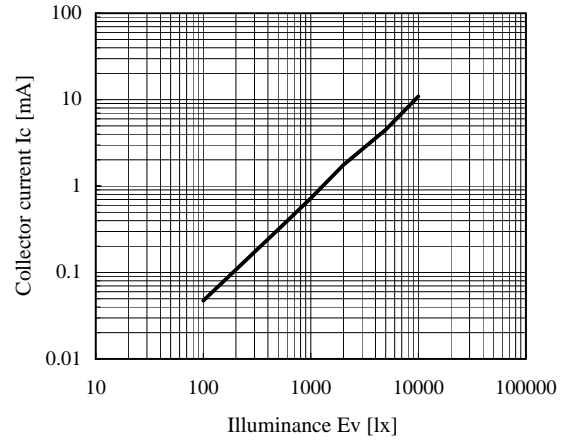
Collector current Vs. Illuminance V_{ce}=5V
