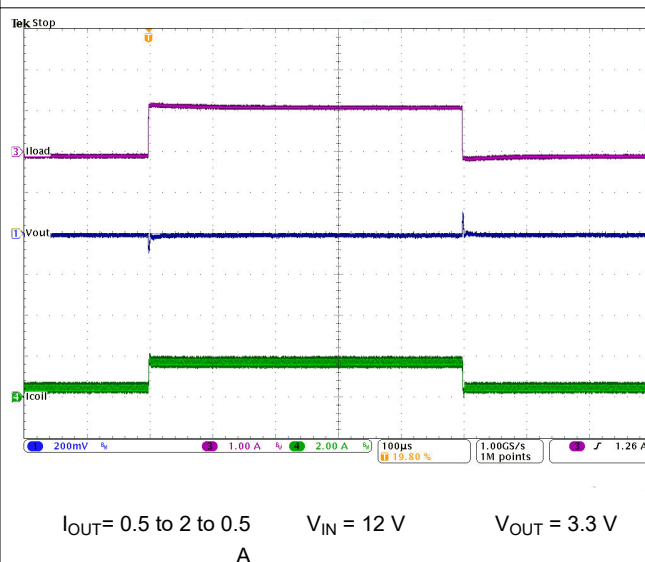
图 9-31. Load Transient Response
