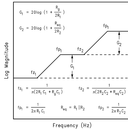
Figure 40. Design Equations
