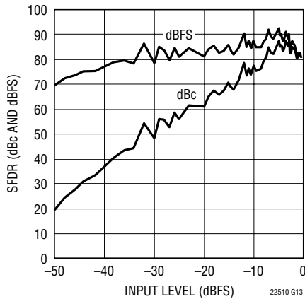
LTC2251: SFDR vs Input Level, f_{IN} = 70\text{MHz} , 2V Range, 125Msps
