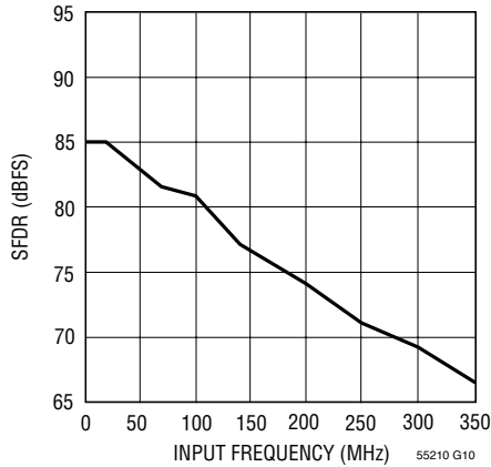
LTC2251: SFDR vs Input Frequency, -1dB, 2V Range, 125Msps
