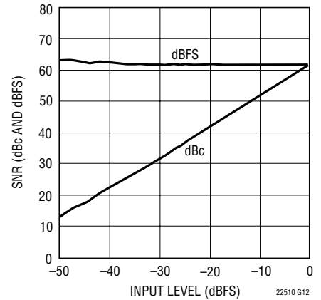
LTC2251: SNR vs Input Level, f_{IN} = 70\text{MHz} , 2V Range, 125Msps
