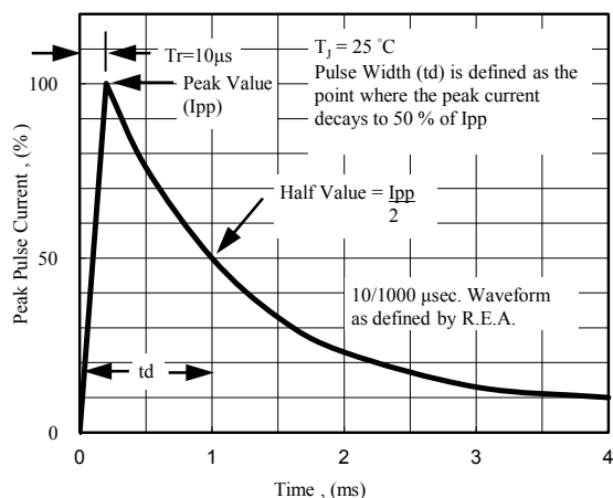
Fig. 5 - Pulse Waveform
